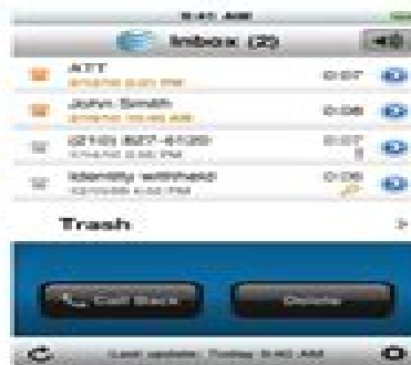
Figure 14: Inbox
