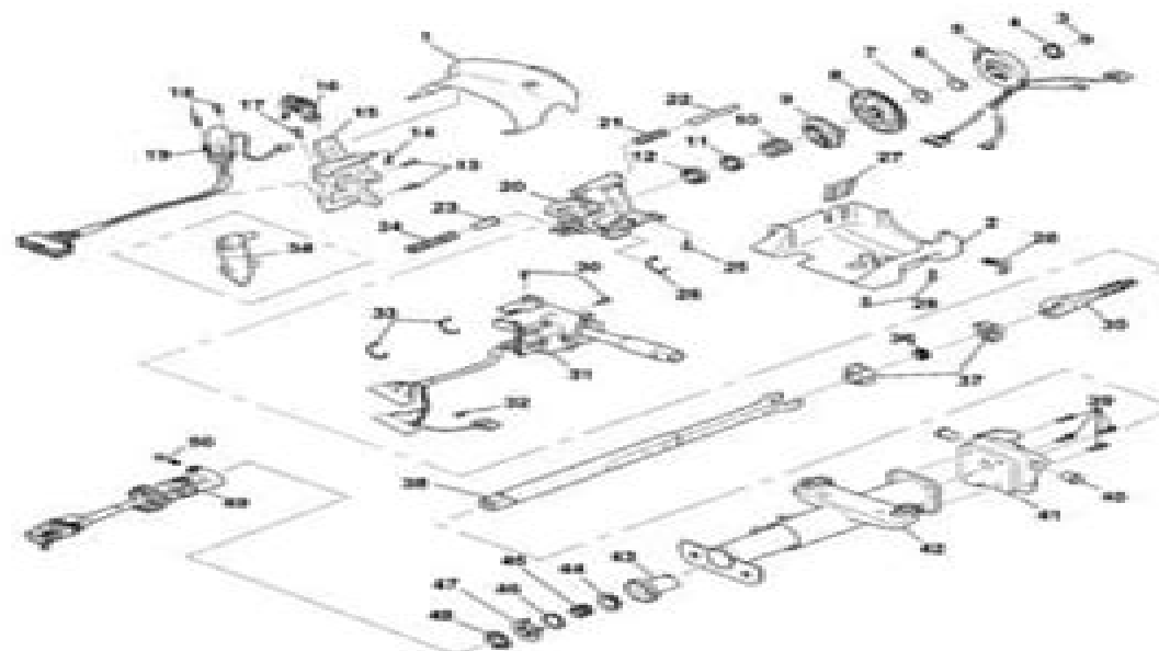
Fig. 1: Tilt Steering Column Disassembled View, Floor Shift Courtesy of GENERAL MOTORS CORP.
