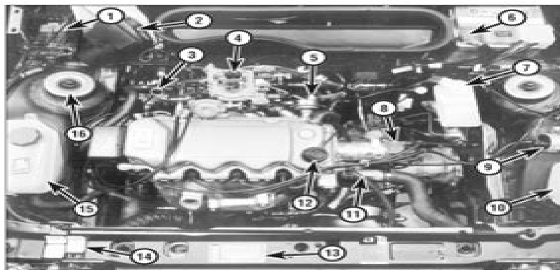
Engine and under bonnet component locations on 1985 RS Turbo models
