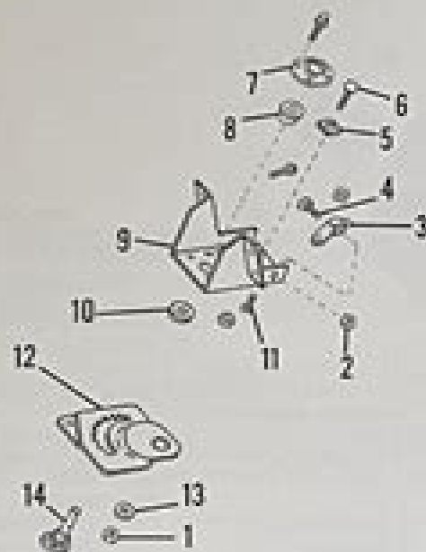
Fig. AR4-4—Exploded view of steering gear. Refer to Fig. AR4-3 for cross-sectional view.
