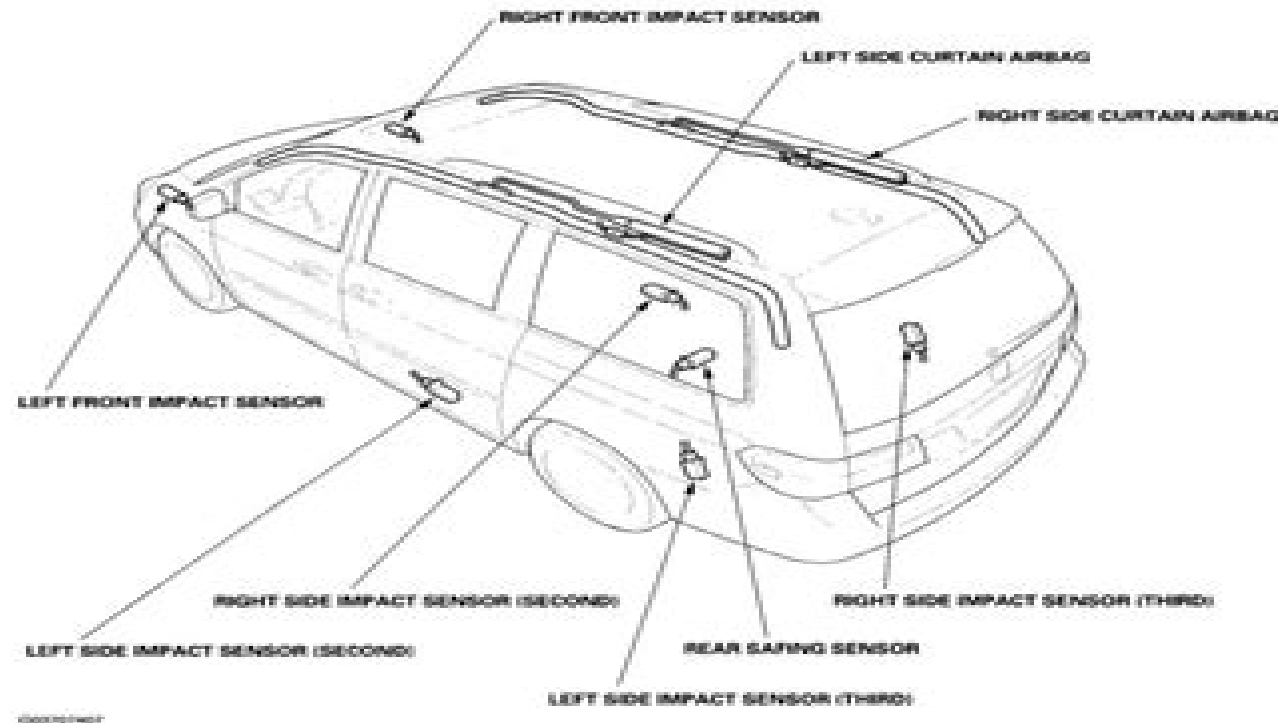
Fig. 2: Identifying SRS Components Location (2 Of 2) Courtesy of AMERICAN HONDA MOTOR CO., INC.
