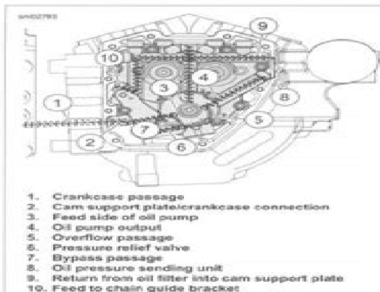
Figure 3-2. Cam Support Plate Oil Flow
