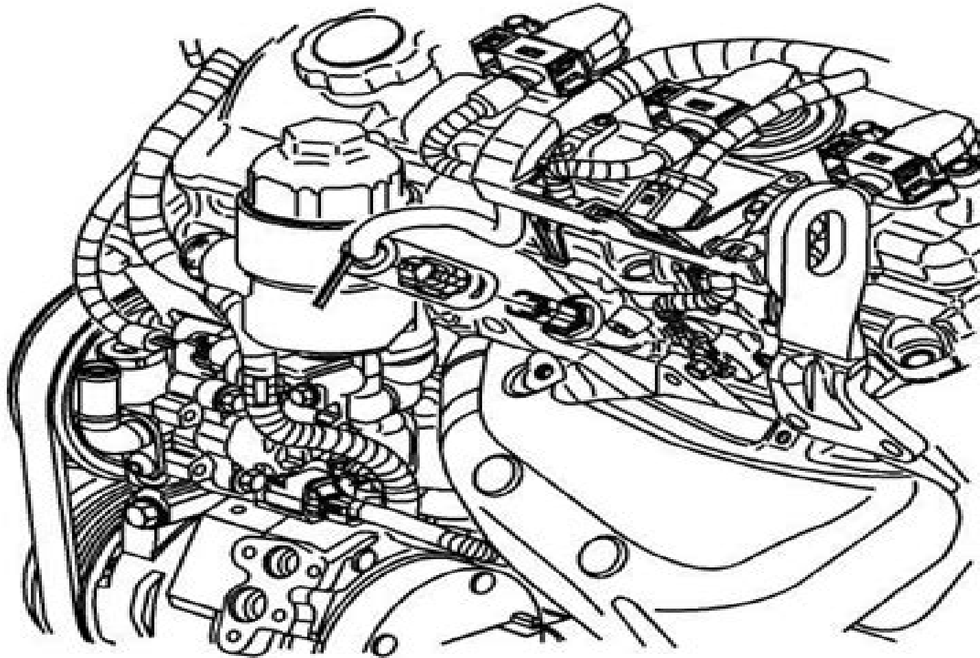
Fig. 43: View Of Coolant Temperature Sensor And Electrical Connector Courtesy of GENERAL MOTORS CORP.
